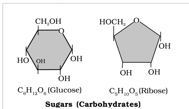
Fig. 9.1 (a) - Sugars (carbohydrates): glucose ( \text{C}_6\text{H}_{12}\text{O}_6 ) and ribose ( \text{C}_5\text{H}_{10}\text{O}_5 ), the small-molecular-weight sugars of living tissue.
