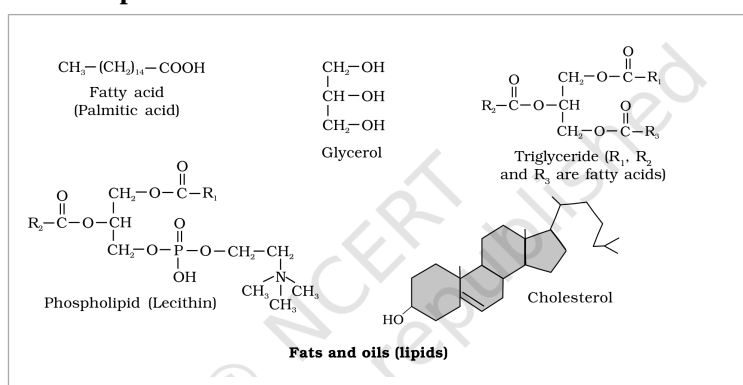
Fig. 9.1 (c) - Fats and oils (lipids): a fatty acid (palmitic acid), glycerol, a triglyceride ( \text{R}_1 , \text{R}_2 , \text{R}_3 are fatty acids), a phospholipid (lecithin) and cholesterol.
